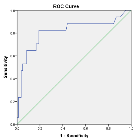
Figure 1. Receiver Operating Characteristic (ROC) curve derived from our study, depicting the diagnostic performance of measured red blood cell count per high-power field (RBC/hpf) in distinguishing between cases with and without detected lesions.
